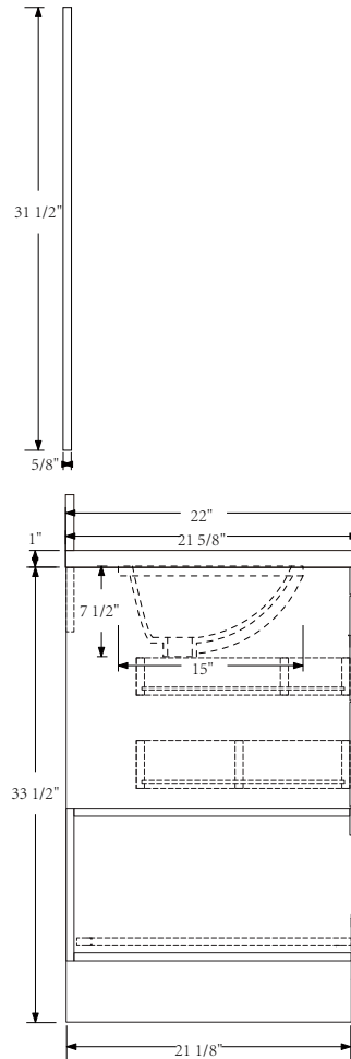
SIDE VIEW
